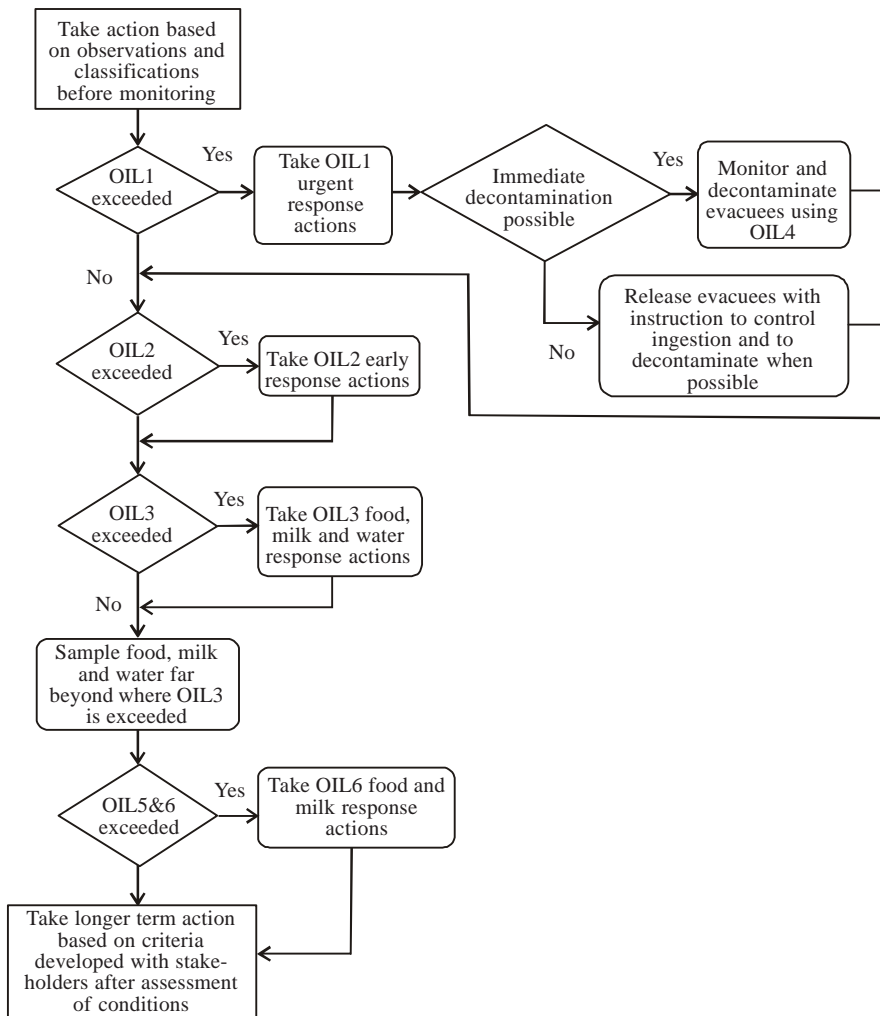
Figure 2 : Process of assessment of a nuclear or radiological emergency resulting in contamination of a large area
