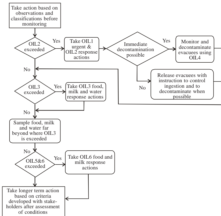
Figure 3 : Process of assessment of a nuclear or radiological emergency resulting in contamination of moderate area
