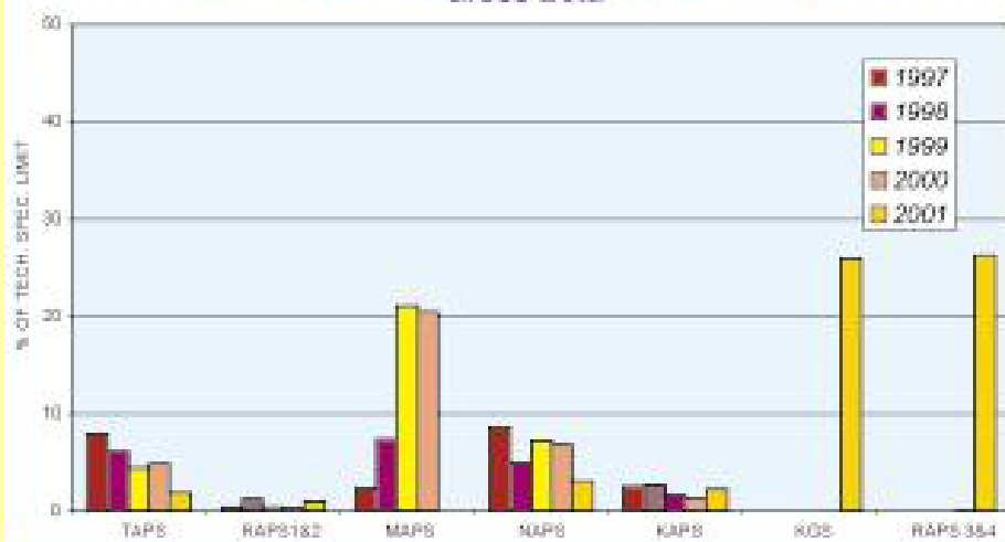
Fig. 2b LIQUID DISCHARGES FROM NPPs Gross Beta
